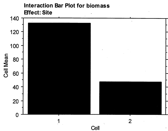
Figure 3: Mean grass biomass per plot by site. Site 1: Restored. Site 2: Remnant.
