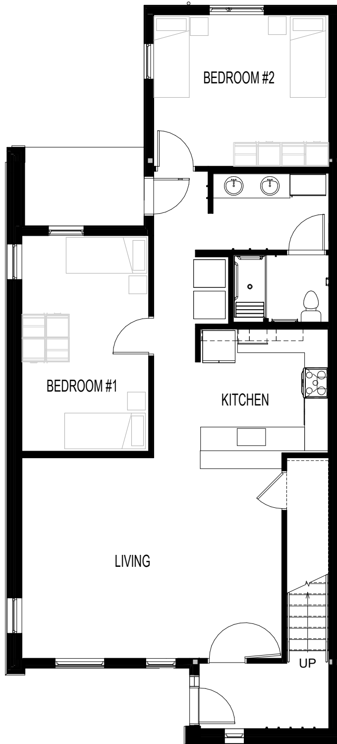
Townhome Level 1
